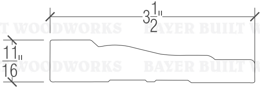
144A Casing
